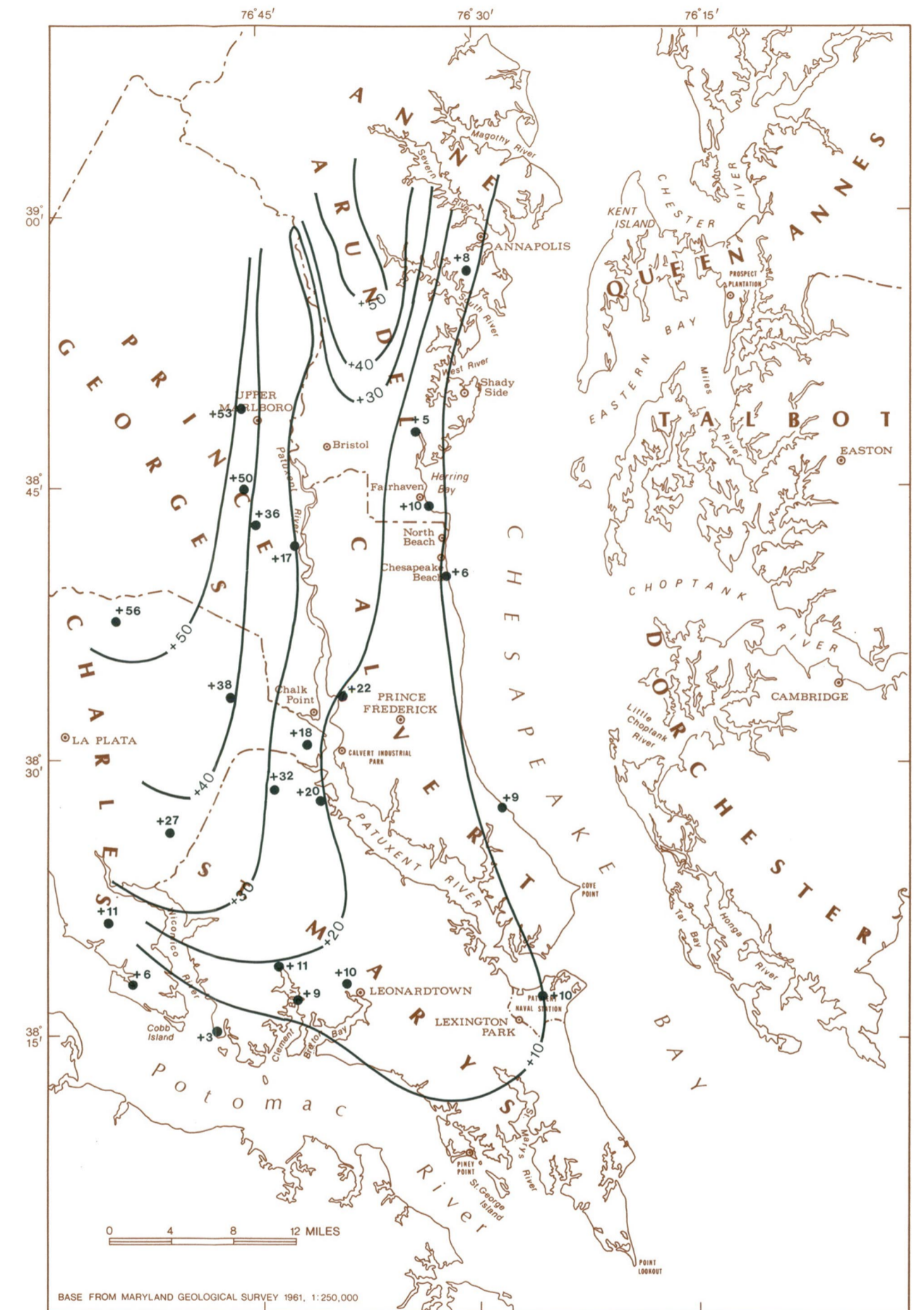
Simulated pre-pumping potentiometric surface and water levels measured early in aquifer development as reported by Darton (1896), Clark and others (1918), and Otton (1955).
