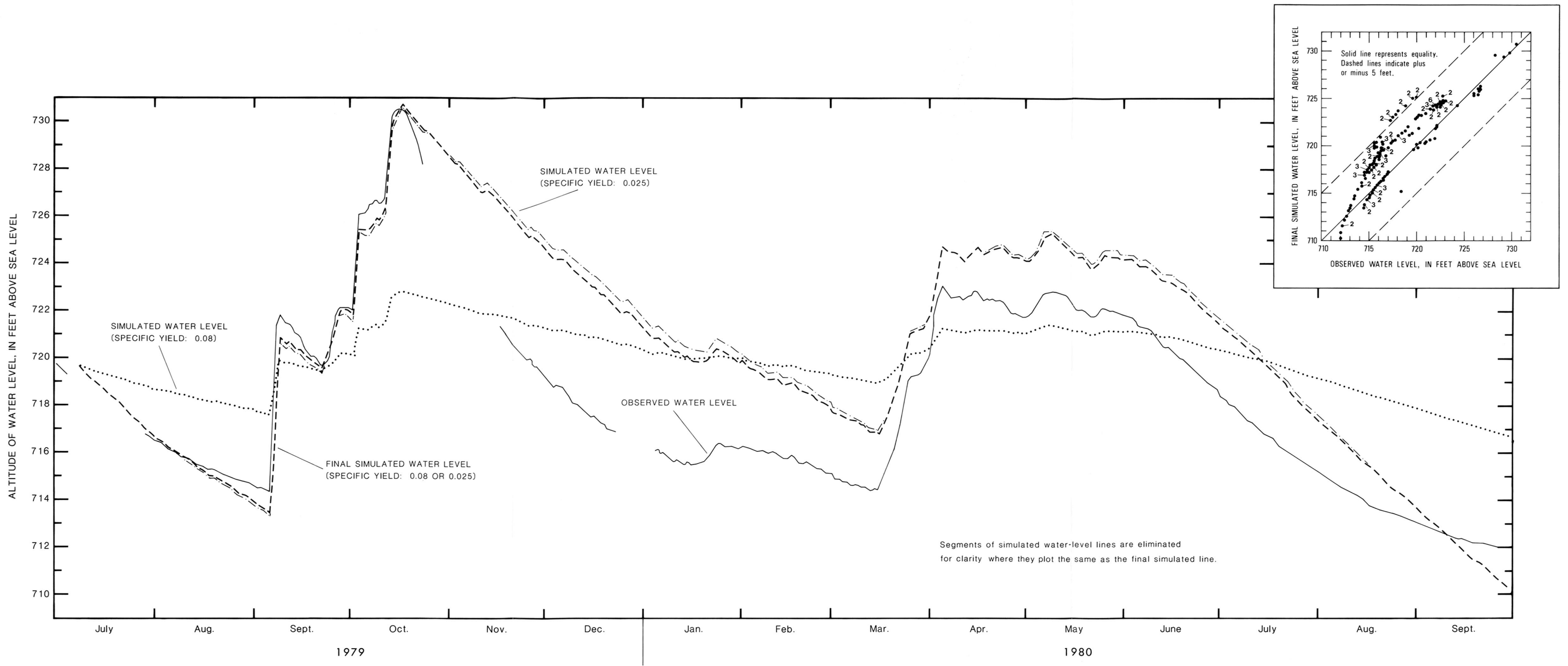
Figure 26. — Simulated water levels, cell B, compared with observed water levels for well HO-BB 26, July 1979 to September 1980.
