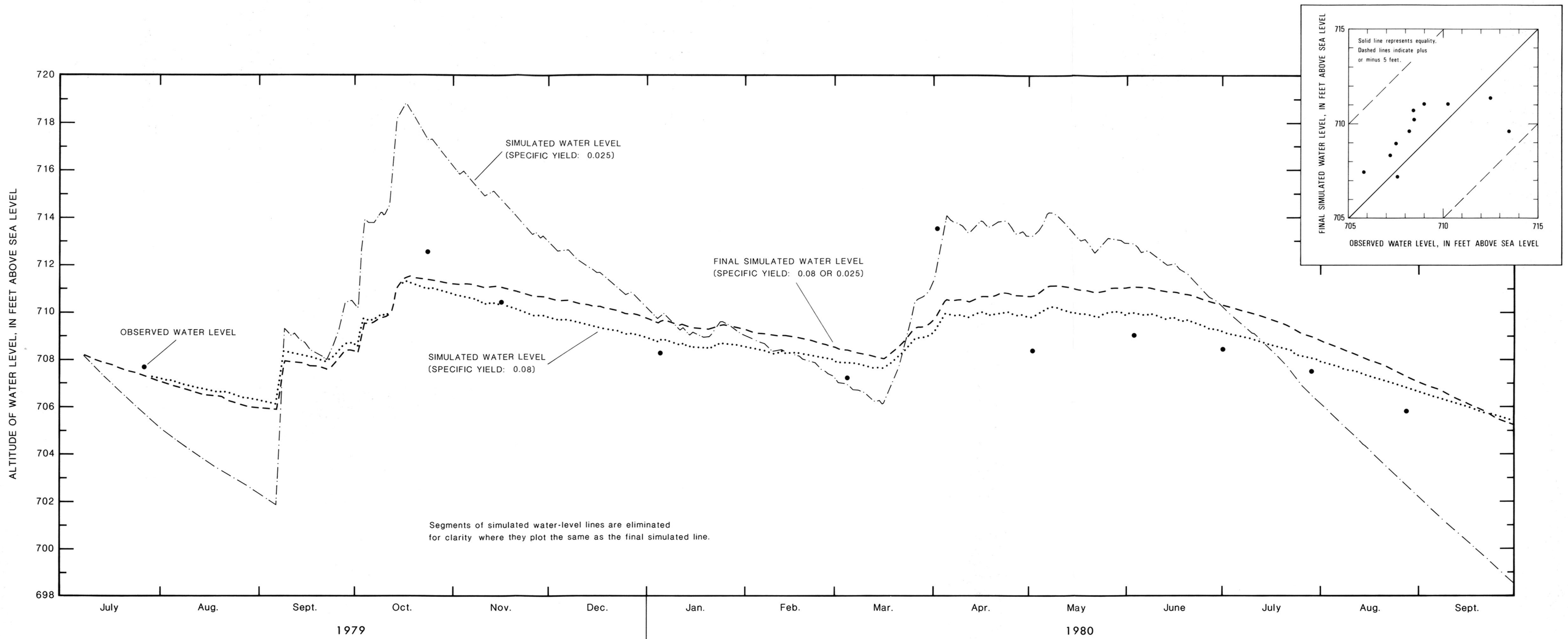
Figure 27. — Simulated water levels, cell A, compared with observed water levels for well HO-AB 4, July 1979 to September 1980.
