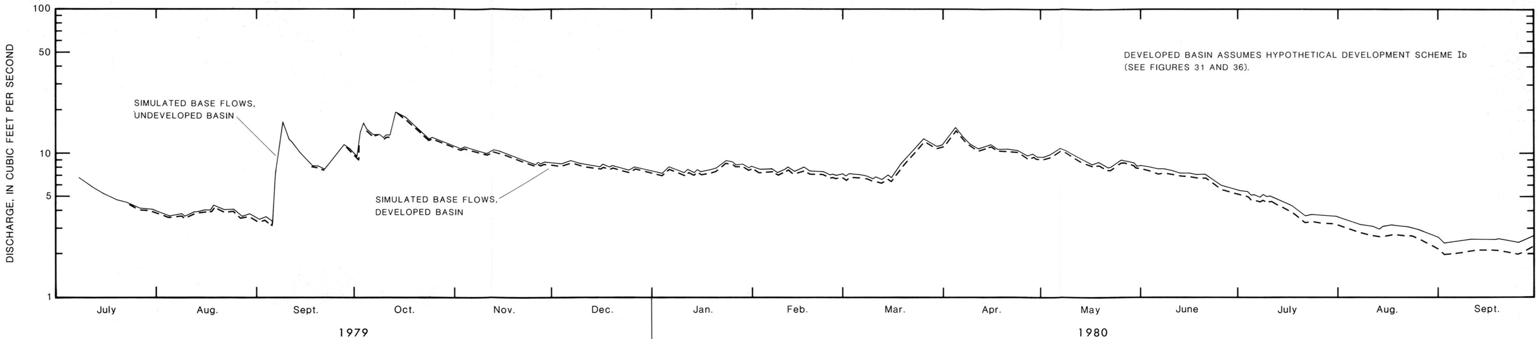
Figure 49. — Comparison of simulated base flows at streamflow site 11 for developed (scheme Ib) and undeveloped basin, July 1979 to September 1980.
